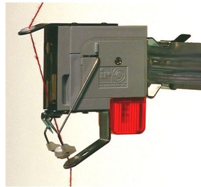
331.000.064.11 UFW 12V / 1,2kOhm with inclined yarn outflow, ball tension and trapper
