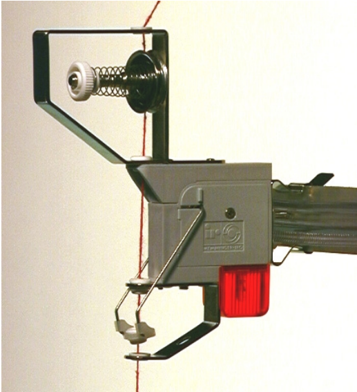
331.000.063.01 UFW 12V / 1,2kOhm with straight yarn outflow and cymbal tension
