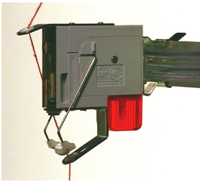
331.000.064.01 UFW 12V / 1,2kOhm with inclined yarn outflow and ball tension
