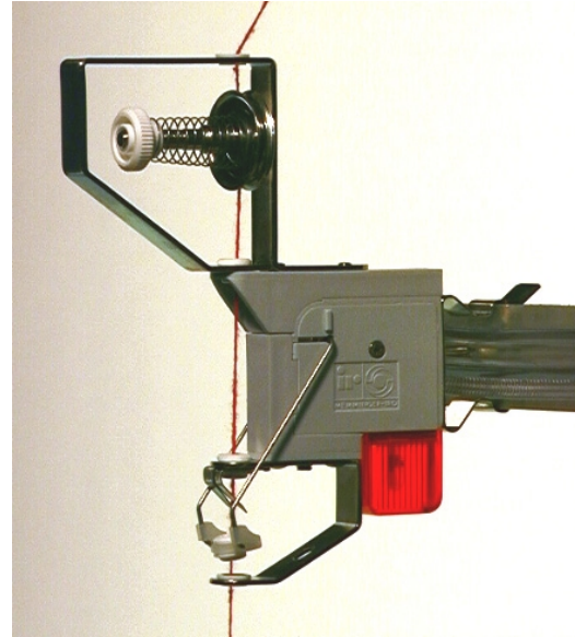
331.000.063.11 UFW 12V / 1,2kOhm with straight yarn outflow, cymbal tension and trapper
